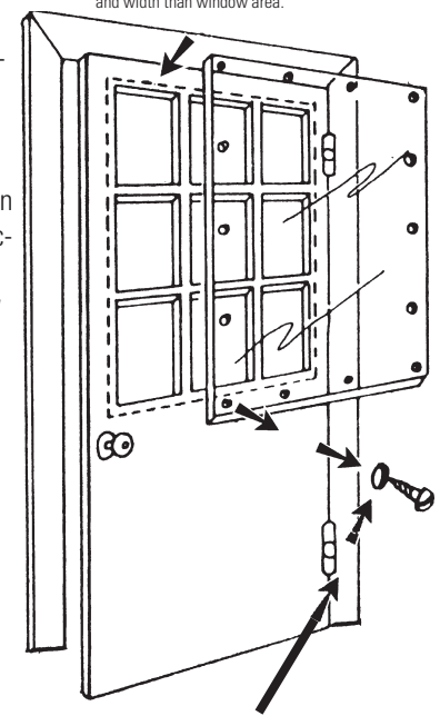
Round-head screws 1/2" in length with finishing washers.
